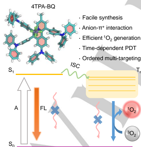
Scheme 1. Illustration of 4TPA-BQ for time-dependent PDT.
