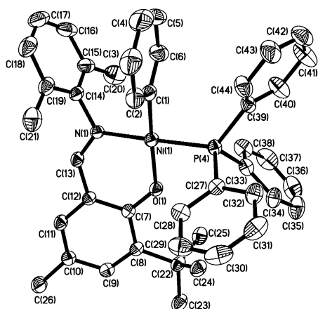
Figure 1. Molecular structure of complex 1 . Selected bond lengths [Å] and angles [deg]: Ni(1)–C(1) = 1.887(3), Ni(1)–O(1) = 1.9126(18), Ni(1)–N(1) = 1.920(2), Ni(1)–P(4) = 2.1731(8), C(1)–Ni(1)–O(1) = 171.43(10), C(1)–Ni(1)–N(1) = 92.62(10), O(1)–Ni(1)–N(1) = 92.25(8), C(1)–Ni(1)–P(4) = 85.24(8), O(1)–Ni(1)–P(4) = 89.75(6).
