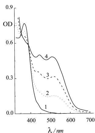
Figure 1. UV/Vis spectrum of 1-( p - tert -butylphenoxy)-2-azidoanthraquinone ( 3b , 1.4 \times 10^{-4} mol L ^{-1} ) before (spectrum 1) and after irradiation at 313 nm for 1 min (spectrum 2), 4 min (spectrum 3) and 16 min (spectrum 4) in toluene at ambient temperature.
