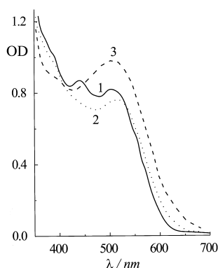
Figure 2. UV/Vis spectrum recorded after 16 min irradiation of 1-( p - tert -butylphenoxy)-2-azidoanthraquinone ( 3b , 2.3 \times 10^{-4} mol L ^{-1} ) in toluene at ambient temperature (spectrum 1), its change after addition of methanol (5% vol.) (spectrum 2), and UV/Vis spectrum recorded after irradiation of 3b for 16 min in toluene in the presence of 0.1 mol L ^{-1} of p - tert -butylphenol (spectrum 3).
