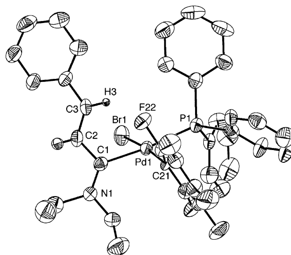
Figure 1. X-ray structure of complex 4 . Selected bond lengths (Å): Pd1–C1, 2.025(6); Pd1–C21, 2.031(6); Pd1–Br1, 2.4844(16); Pd1–P1, 2.324(2); C1–C2, 1.467(9); C1–N1, 1.300(8); C2–C3, 1.330(10).
