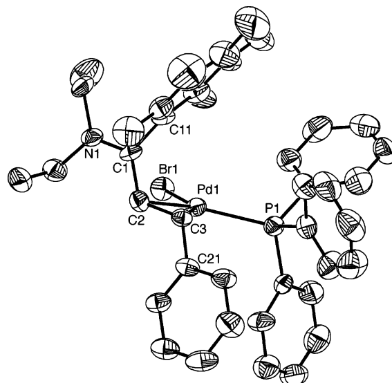
Figure 2. X-ray structure of complex 7 . Selected bond lengths (Å): Pd1–C2, 2.167(13); Pd1–C3, 2.095(12); Pd1–Br1, 2.5456(16); Pd1–P1, 2.278(3); C1–N1, 1.335(13); C1–C2, 1.413(15); C2–C3, 1.416(15).
