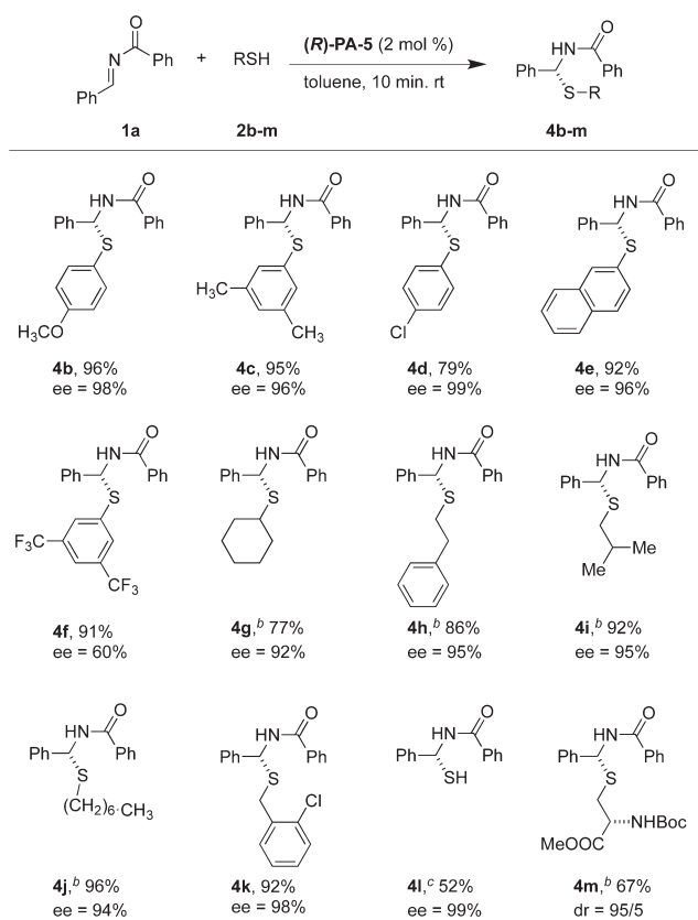
Scheme 1. Catalytic Asymmetric Addition of Thiols to N -Acyl Imines a
