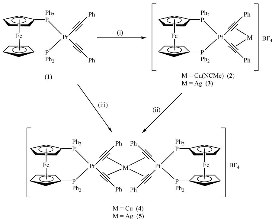
Scheme 1. (i) 1 equivalent [\text{Cu}(\text{NCMe})_4]\text{BF}_4 or \text{AgBF}_4 , \text{CHCl}_3\text{--MeCN} . (ii) \text{CH}_2\text{Cl}_2\text{--hexane} , room temperature. (iii) 0.5 equivalent [\text{Cu}(\text{NCMe})_4]\text{BF}_4 or \text{AgBF}_4 , \text{CHCl}_3\text{--MeCN} .
