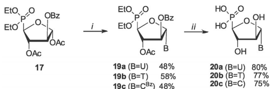
SCHEME 3 Preparation of nucleoside phosphonates with D- threo configuration
