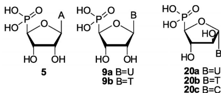
FIG. 4 The NMR-evaluated β-D-erythrose ( 5 , 9a , 9b ) and α-D-threose ( 20a–20c ) nucleotide analogues
