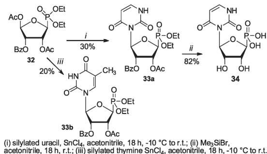
SCHEME 5 Preparation of nucleoside phosphonate with L -erythro configuration
