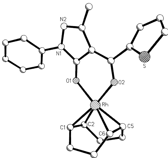
Fig. 2. Molecular structure of derivative 1.
