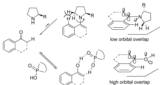
Figure 1. Phosphoric acid catalysis versus enamine catalysis.
