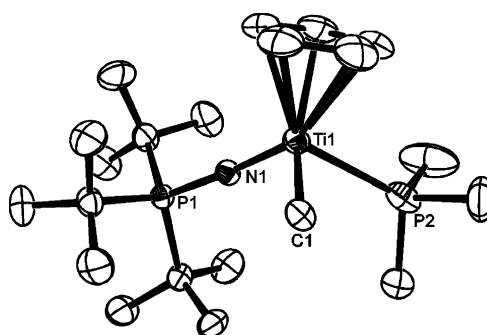
Figure 1. ORTEP drawing of the cation of 17 ; 30% thermal ellipsoids are shown. Hydrogen atoms are omitted for clarity. Distances (Å) and angles (deg): Ti(1)–N(1) 1.769(3), Ti(1)–C(1) 2.193(3), Ti(1)–P(2) 2.6723(18), P(1)–N(1) 1.618(3), N(1)–Ti(1)–C(1) 102.16(12), N(1)–Ti(1)–P(2) 105.08(9), C(1)–Ti(1)–P(2) 92.02(10), P(1)–N(1)–Ti(1) 172.2(2).
