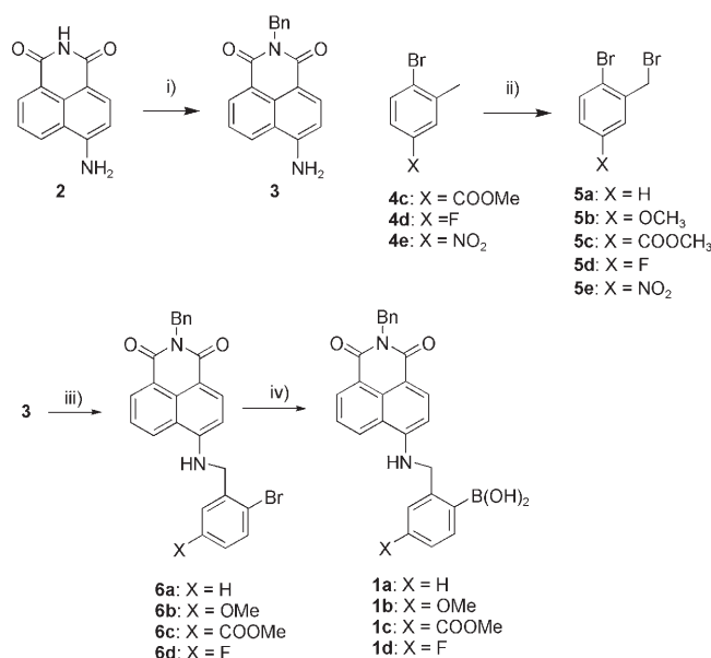
Scheme 2. a) \text{NaOCH}_3/\text{CH}_3\text{OH} , BnBr, DMF, room temperature; b) NBS, AIBN, \text{CCl}_4 , reflux, h\nu ; c) NaH, DMF, 5a–d , room temperature; 4) neopentylglycol diboron, [\text{PdCl}_2(\text{dppf})] , KOAc, DMSO, 90^\circ\text{C} . DMF: N,N -dimethylformamide; NBS: N -bromosuccinimide; AIBN: azobisisobutyronitrile; dppf: 1,1'-bis(diphenylphosphanyl)ferrocene; DMSO: dimethylsulfoxide.
