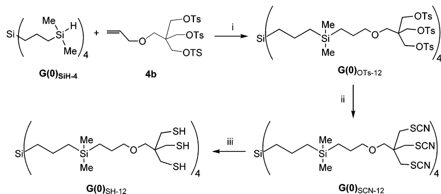
Scheme 4. Attachment of a Tripod Ligand Precursor to Carbosilane Dendrimers a
