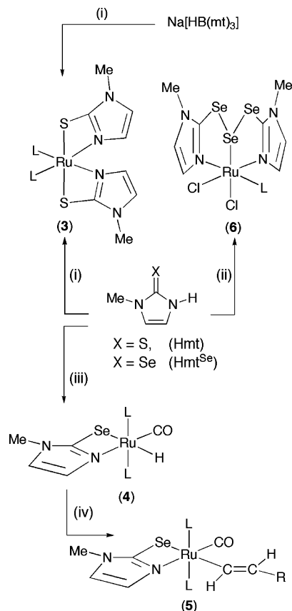
Scheme 1. Synthesis of Methimazolyl, Selenomethimazolyl, and Triselenane Complexes ( L = PPh_3 ) a
