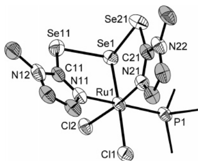
Figure 2. Molecular geometry of 6 in a crystal of 6 \cdot (CH_2Cl_2)_2 (50% displacement ellipsoids, phenyl groups and hydrogen atoms omitted). Selected bond distances (Å) and angles (deg): Ru1–N21 2.062(6), Ru1–N11 2.112(5), Ru1–Se1 2.2998(10), Ru1–P1 2.3333(18), Ru1–Cl1 2.4241(18), Ru1–Cl2 2.4439(17), Se1–Se21 2.4161(11), Se1–Se11 2.4311(11), Se11–C11 1.879(7), Se21–C21 1.876(8), N21–Ru1–N11 83.7(2), N21–Ru1–Se1 91.14(16), N11–Ru1–Se1 88.71(17), N21–Ru1–P1 92.00(16), Se1–Ru1–P1 94.82(5), N21–Ru1–Cl1 91.23(17), N11–Ru1–Cl1 90.15(17), P1–Ru1–Cl1 86.51(6), Se1–Ru1–Cl2 86.86(5), P1–Ru1–Cl2 95.49(6), Cl1–Ru1–Cl2 90.61(6), Ru1–Se1–Se21 102.73(4), Ru1–Se1–Se11 101.82(4), Se21–Se1–Se11 104.44(4), C11–Se1–Se1 91.9(2), C21–Se21–Se1 93.3(2).
