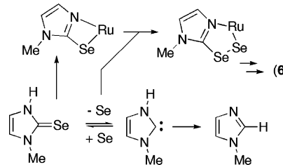
Scheme 2. Possible Decomposition Routes for Hmt^{Se}
