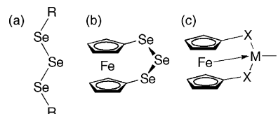
Chart 1. (a) Diorganotriselenanes; (b) Triselenoferrocenophane; (c) Metalladichalcaferrocenophanes ( \text{X} = \text{S}, \text{Se}; \text{M} = \text{Pd}, \text{Pt}; \text{L} = \text{PPh}_3 ) 2c,3
