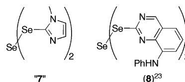
Scheme 2. Possible Decomposition Routes for Hmt^{Se}
