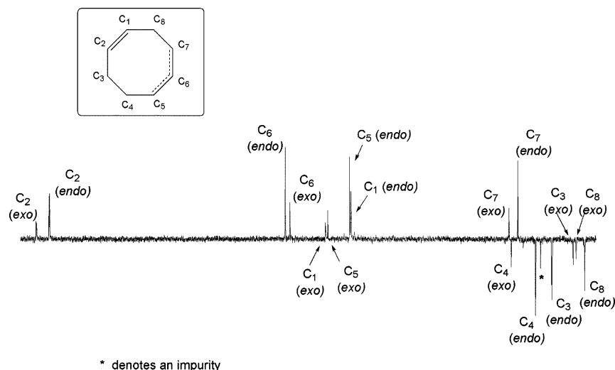
Figure 5. J -modulated ^{13}\text{C}\{^1\text{H}\} NMR spectrum for endo-3 and exo-3 obtained at 245 K in toluene- d_8 highlighting the cyclooctadienyl carbon resonances. The CH resonances point up and the \text{CH}_2 resonances point down. The spectral range indicated is from \delta 110 for \text{C}_2 ( exo ) to \delta 25 for \text{C}_8 ( endo ).
