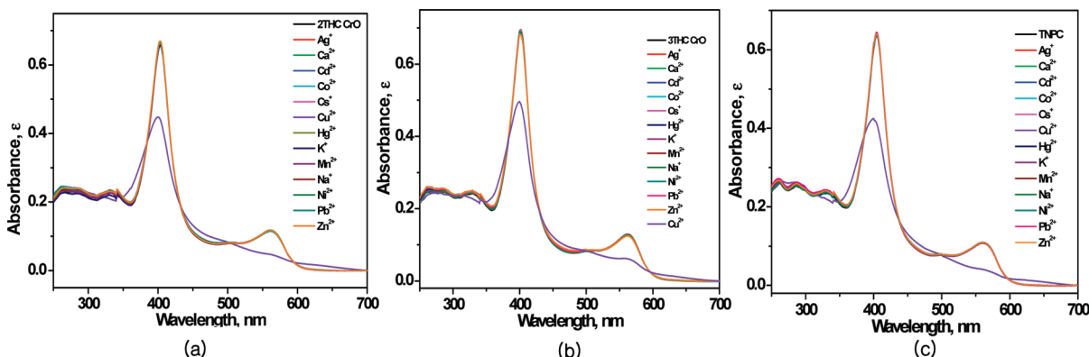
Figure 6. Changes of the absorption spectra of (a) 1a , (b) 2a , and (c) 3a upon the addition of various metal ions. The ligand/metal ion ratio is 1:1. The concentration of the ligand in CH 2 Cl 2 is 1 \times 10^{-5} M, and that of the M^{n+} solution in CH 3 CN is 1 \times 10^{-3} M.
