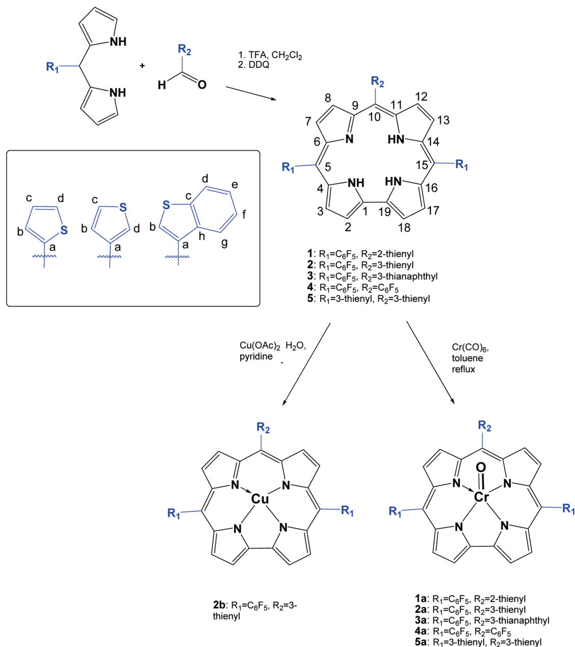
Scheme 2. Synthesis of A 2 B-metalloporphyrins from Commercially Available Starting Materials
