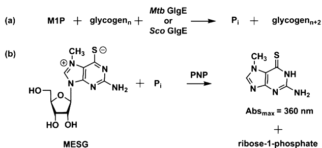
Figure 2. GlgE-coupled enzyme assay utilizing PNP; (a) M1P and glycogen ( n = a number of maltose units) serve as substrates for GlgE; (b) PNP consumes \text{P}_i and MESG to form 2-amino-6-mercaptopurine.
