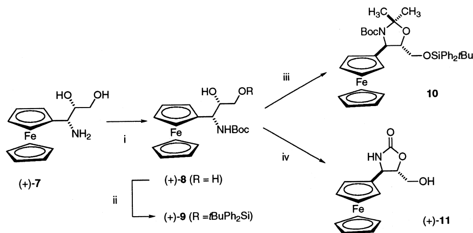
Scheme 3. Reagents and conditions: (i) 1.2 equivalents Boc 2 O, three equivalents NaHCO 3 , MeOH, ultrasound, r.t., 2 h, 78%; (ii) 2.2 equivalents imidazole, 1.1 equivalents t BuPh 2 SiCl, DMF, r.t., 24 h, 89%; (iii) 10 equivalents (MeO) 2 CMe 2 , cat. p TsOH, benzene, reflux, 5.5 h, 69%; (iv) 2.5 equivalents NaH, DMF, r.t., 1.5 h; 1 M aq. HCl, r.t., 83%.
