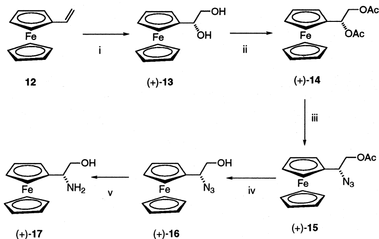
Scheme 4. Reagents and conditions: (i) three equivalents K 3 [Fe(CN) 6 ], three equivalents K 2 CO 3 , 0.1 equivalents (DHQD) 2 PYR, 0.1 equivalents K 2 OsO 2 (OH) 4 , CH 3 CN–water (1:1), r.t., 12 h, 79% (98% ee); (ii) nine equivalents Ac 2 O, pyridine, r.t., 12 h, 97%; (iii) 5.5 equivalents NaN 3 , MeOH–water (1:3), r.t., 12 h, 72%; (iv) 2.5 equivalents DIBAL-H, diethyl ether, –78 °C, 1 h, 97%; (v) H 2 (1 atm), cat. 10% Pd/C, ethyl acetate, r.t., 12 h, 100%.
