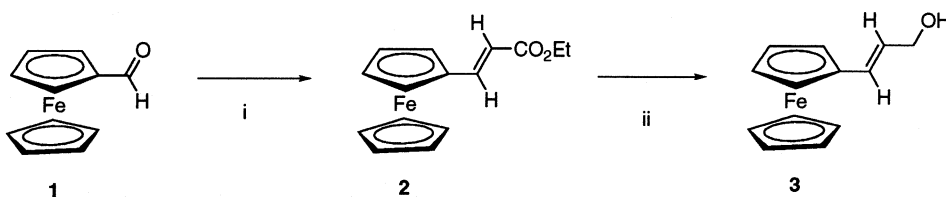
Scheme 1. Reagents and conditions : (i) three equivalents (EtO) 2 PO–CH 2 –CO 2 Et, two equivalents NaH, benzene, 60 °C, reflux, 20 h, 97%; (ii) 2.4 equivalents DIBAL-H, diethyl ether, –75 °C, 2 h, –20 °C, 1 h, 87%.
