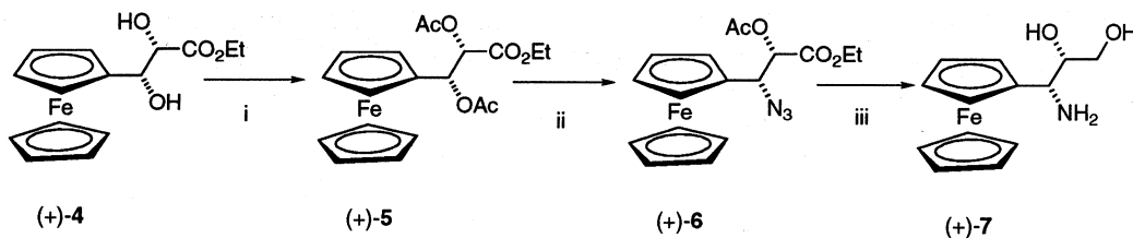
Scheme 2. Reagents and conditions : (i) 11 equivalents Ac 2 O, pyridine, r.t., 17 h, 98%; (ii) six equivalents NaN 3 , MeOH–water (1:3), r.t., 66 h, 77%; (iii) seven equivalents LAH, THF, reflux, 3.5 h, 83%.
