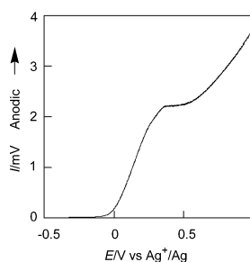
Figure 1. Linear sweep voltammogram of 1 (2 mM) in the presence of DB24C8 (4 mM) in acetonitrile solution of 10 mM n -Bu 4 NPF 6 .
