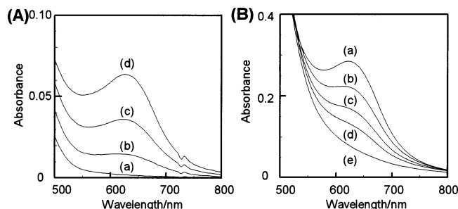
Figure 3. UV-vis spectra of 1 in the presence of DB24C8 in \text{CH}_3\text{CN} solution of 10 mM n\text{-Bu}_4\text{NPF}_6 . [\mathbf{1}]_0 = 2.0 mM, [\text{DB24C8}]_0 = 4.0 mM. (A) Spectra measured immediately after the electrolysis at (a) -0.4 V (vs \text{Ag}^+/\text{Ag} ), (b) 0 V, (c) 0.05 V, (d) 0.1 V. (B) Change in the spectra by flow electrolysis at 0.4 V (293 K) and subsequent reactions. (a) 0 min, (b) 6 min, (c) 12 min, (d) 24 min, and (e) 90 min after electrolysis.
