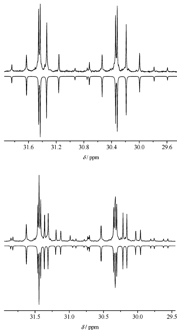
Figure 5. ^{31}\text{P}\{^1\text{H}\} NMR spectra of (\text{PPh}_3)_3\text{Rh}^{14}\text{NCB}(\text{CF}_3)_3 (upper traces) and (\text{PPh}_3)_3\text{Rh}^{15}\text{NB}(\text{CF}_3)_3 (lower traces); simulated spectra ( g\text{NMR} ) inverted.
