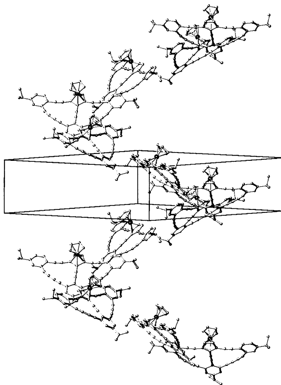
Fig. 3. Packing diagram of 12 . Visible is the 6-fold axis in that the single molecules of 12 are packed in the solid state.
