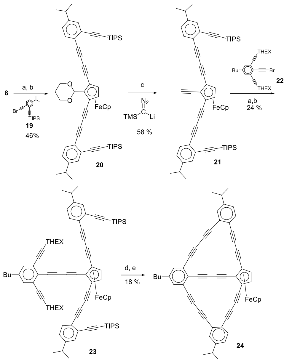
Scheme 4. (a) BuLi, then CuI 15 min; (b) propylamine, 19 , 22 °C, 1 h; (c) TsOH, 1 h 22 °C; (d) tetrabutylammonium fluoride, THF, 24 °C, 1 h; (e) \text{Cu}(\text{OAc})_2 , \text{CH}_3\text{CN} , 80 °C, 8 h.
