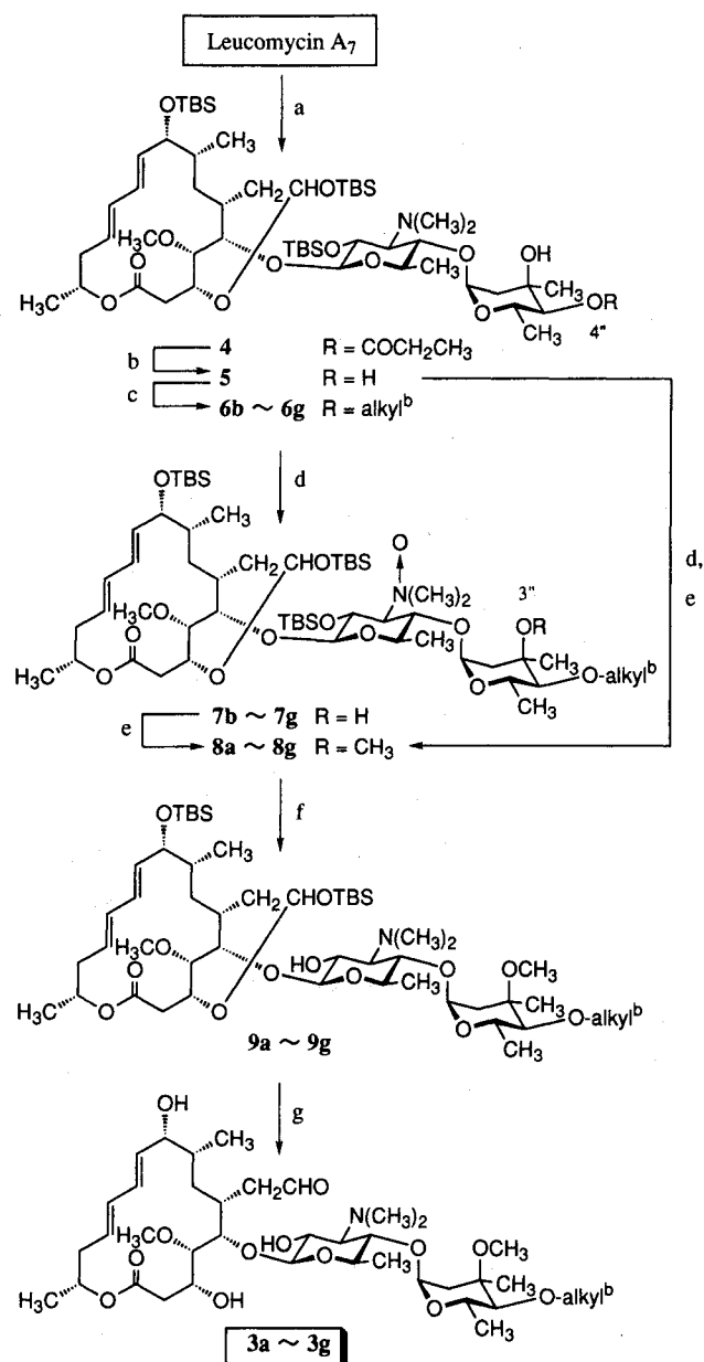
Scheme 1. Synthesis of compounds 3a ~ 3g a,b .
