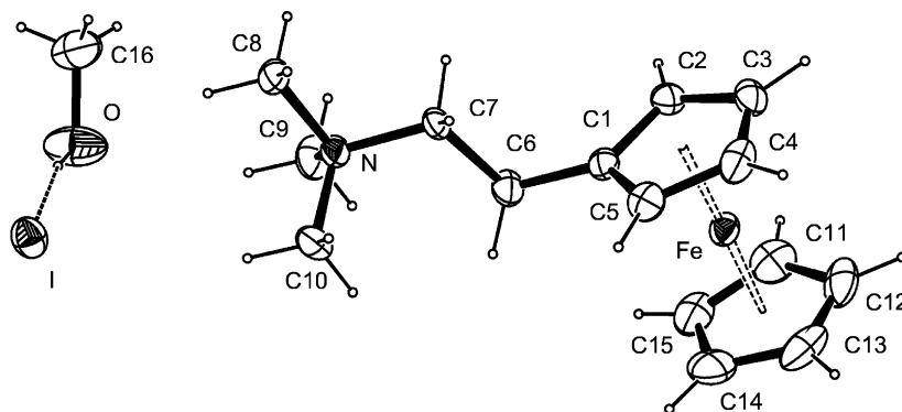
Fig. 3. Molecular structure of [\text{Fe}(\text{C}_5\text{H}_5)(\text{C}_5\text{H}_4\text{CH}_2\text{CH}_2\text{NMe}_3)]\text{I} \cdot \text{MeOH} ( XIII ), showing the atom numbering scheme; the picture was drawn with the use of the ORTEP program.
