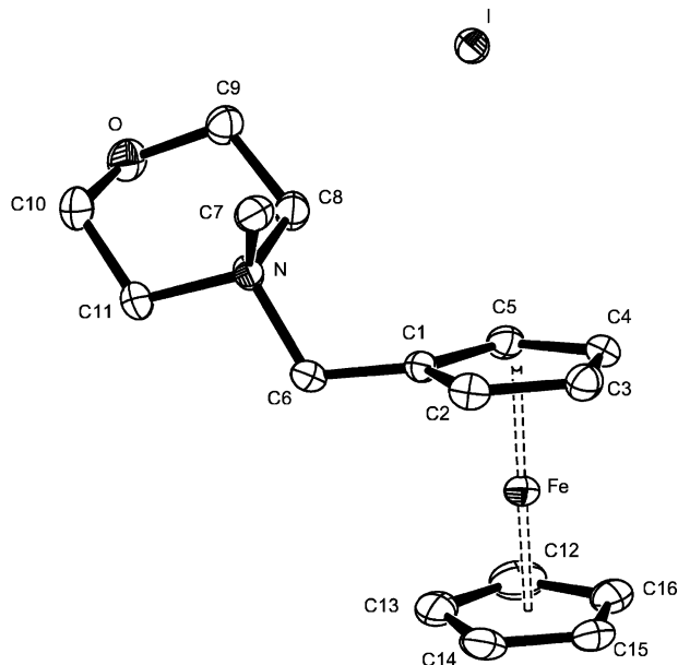
Fig. 4. Molecular structure of [\text{Fe}(\text{C}_5\text{H}_5)(\text{C}_5\text{H}_4\text{CH}_2\text{NMeC}_4\text{H}_8\text{O})]\text{I} ( XIV ), showing the atom numbering scheme; the picture was drawn with the use of the ORTEP program.
