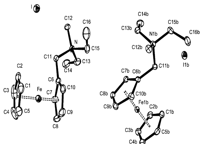
Fig. 2. Molecular structure of [\text{Fe}(\text{C}_5\text{H}_5)(\text{C}_5\text{H}_4\text{CH}_2\text{NMeEt}_2)]\text{I} ( XII ), showing the atom numbering scheme; there are two independent molecules differing only in the conformation about the N–C(11) bond; the picture was drawn with the use of the ORTEP program.
