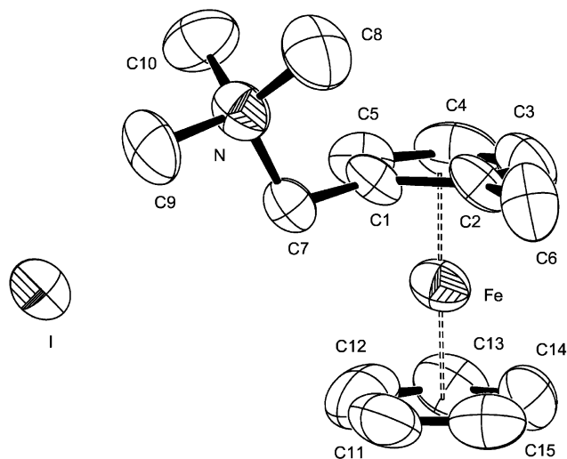
Fig. 1. Molecular structure of [\text{Fe}(\text{C}_5\text{H}_5)\{\text{C}_5\text{H}_3\text{Me}(\text{CH}_2\text{NMe}_3)\}]\text{I} ( VI ), showing the atom numbering scheme; the picture was drawn with the use of the ORTEP program.
