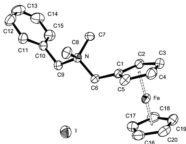
Fig. 5. Molecular structure of [\text{Fe}(\text{C}_5\text{H}_5)(\text{C}_5\text{H}_4\text{CH}_2\text{NMe}_2\text{CH}_2\text{Ph})]\text{I} (XV), showing the atom numbering scheme; the picture was drawn with the use of the ORTEP program.
