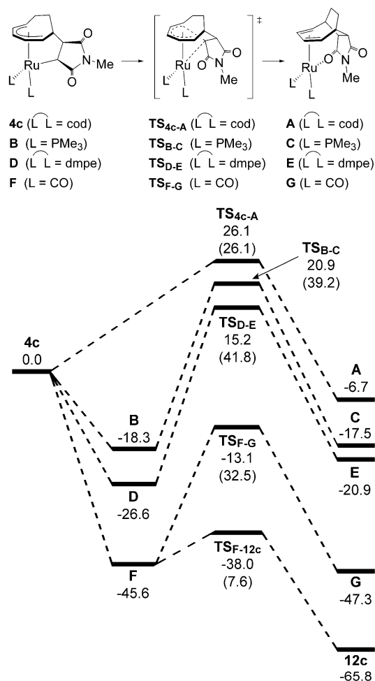
Figure 3. Energy profile for reductive elimination from 4c , B , D , and F to A , C , E , and G , and for the formation of tricarbonyl complex 12c from F . The values in parentheses show net activation energies for the respective steps.
