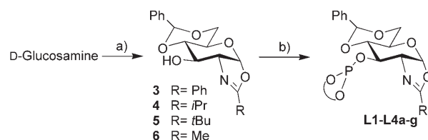
Scheme 3. Synthesis of phosphite-oxazoline ligand library L1–L4a–g . a) Ref. 7. b) 1 equiv of ClP(OR) 2 /Toluene/Py at 80 °C.
