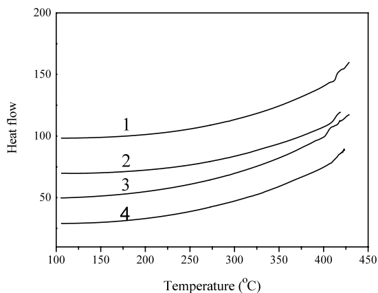
Fig. 5. The glass transition temperature ( T_g ) of polymers by DSC with a heating rate of 20 °C min −1 . 1 , 2 , 3 , and 4 correspond to entries 5, 6, 7, and 8 in Table 3, respectively.
