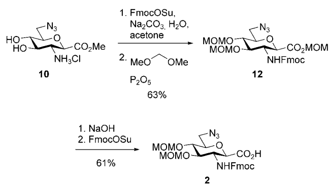
Scheme 2. Synthesis of SDA 2 .
