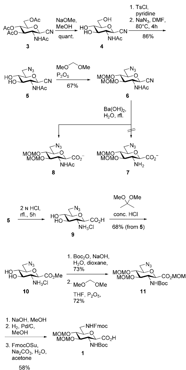
Scheme 1. Synthesis of SDA 1 ; r.f. = reflux.
