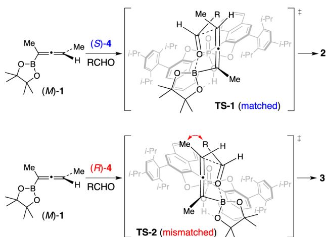
Scheme 4. Transition-State Analysis of the Double Asymmetric Allenylboration Reactions
