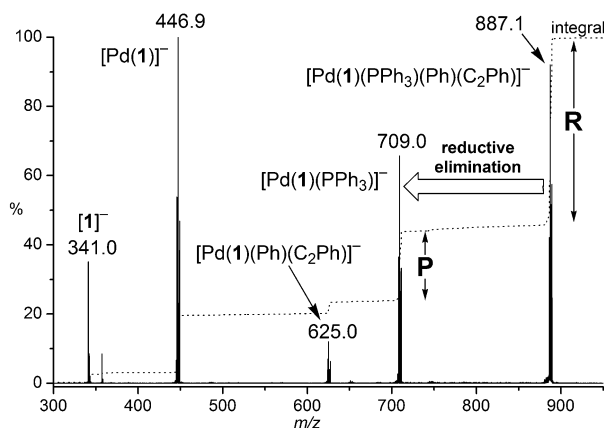
Fig. 3 Negative-ion ESI-MS/MS of [\text{Pd}(\text{I})(\text{PPh}_3)(\text{Ph})(\text{C}_2\text{Ph})]^- , showing reductive elimination of \text{PhC}_2\text{Ph} , at a collision voltage of 15 V.
