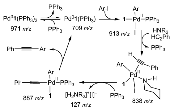
Scheme 1 Intermediates directly observed by negative-ion ESI-MS. Free iodide is also observed.
