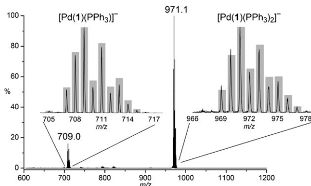
Fig. 1 Negative-ion ESI-MS of Pd(PPh_3)_4 + [PPN][I] in CH_2Cl_2 . Insets: isotope pattern matching for [Pd(PPh_3)_n(I)]^- ( n = 1 and 2 ).
