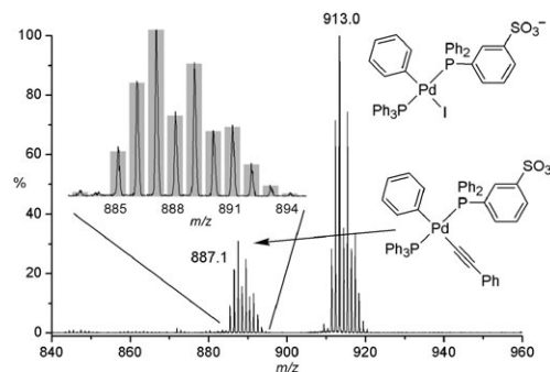
Fig. 2 Negative-ion ESI-MS of Pd(PPh_3)_4 + [PPN][I] + 100 \times (PhI + PhC_2H + NEt_3) in CH_2Cl_2 . Inset: isotope pattern match for [Pd(I)(PPh_3)(Ph)(C_2Ph)]^- .
