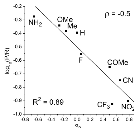
Fig. 4 Plot of \log_{10}(\text{P}/\text{R}) vs. Hammett \sigma_p parameter.
