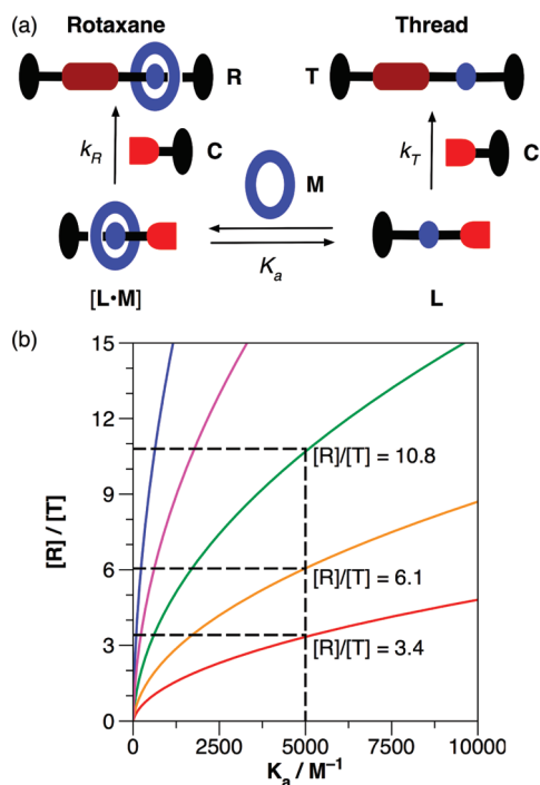
Figure 1. (a) The linear component of the rotaxane L associates with macrocycle M to form the complex [L•M] . This complex is then captured irreversibly by reaction with C to form rotaxane R . The linear component L can also react directly with the capping reagent C , forming T , which does not contain the macrocycle. (b) Plot of [R]/[T] against K_a for the kinetic scheme described in part (a). In the simulation, the starting concentrations of L , M , and C were 25 mM. Rate constant k_T was 1 \times 10^{-3} \text{ M}^{-1} \text{ s}^{-1} , and k_R was varied from 4 \times 10^{-3} \text{ M}^{-1} \text{ s}^{-1} (blue line) to 2.5 \times 10^{-4} \text{ M}^{-1} \text{ s}^{-1} (red line), the value of k_R being halved in each step.
