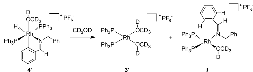
Figure 2. Scheme showing the species generated in a \text{CD}_3\text{OD} solution of 4 (or 4' ).
