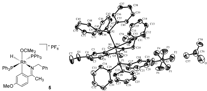
Figure 3. Structural and ORTEP diagram of [\text{Rh}(\text{H})\{\text{PhCH}_2\text{N}=\text{C}(\text{Me})(o\text{-C}_6\text{H}_3\text{-}p\text{-OMe})\}(\text{PPh}_3)_2(\text{acetone})]\text{PF}_6 \cdot \text{Me}_2\text{CO} ( 5 ) with 50% probability thermal ellipsoids.
