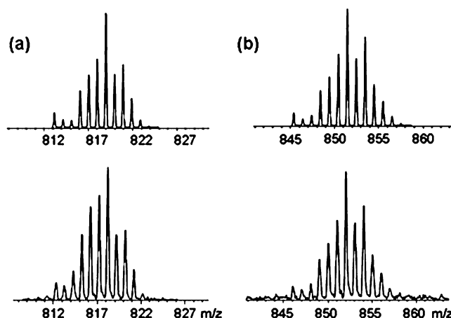
Figure 2. MALDI-MS spectra (anthracene matrix), showing simulated (top) and observed (bottom) isotope patterns for \text{M}^{+\bullet} within (a) 7a (observed m/z 818.3, calculated m/z 818.1); (b) 7b (observed m/z 852.0, calculated m/z 852.1).
