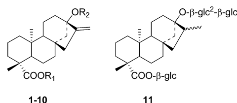
Figure 1. Chemical structure of steviol glycosides 1–10 ( R_1 and R_2 refer to Table 1) and 16,17-dihydrostevioside (11).
