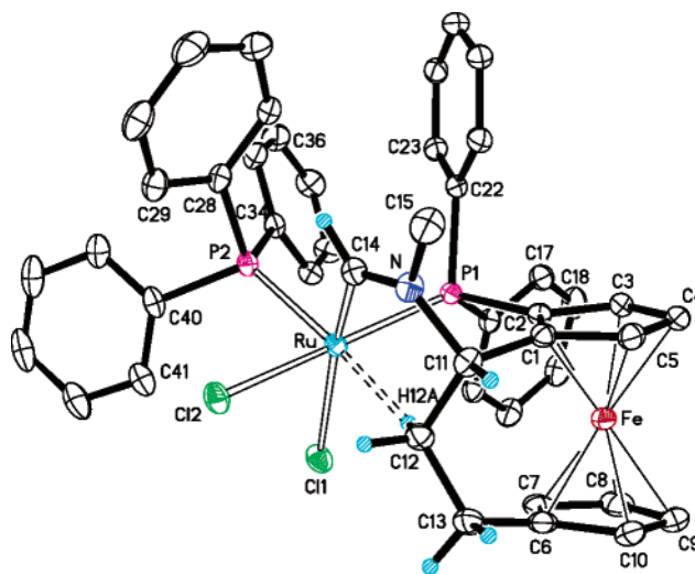
Figure 2. Structural view of 2 showing 30% displacement ellipsoids (aromatic and CH_3 hydrogen atoms and CH_2Cl_2 molecules omitted for clarity). Selected bond lengths and angles ( \text{\AA} , deg): Ru–C(14) 1.957(3), Ru–P(1) 2.349(1), Ru–P(2) 2.267(1), Ru–Cl(1) 2.509(1), Ru–Cl(2) 2.475(1), Ru–C(12) 2.644(3), Ru–H(12a) 1.919, P(2)–Ru–C(14) 93.26(8), P(2)–Ru–P(1) 100.01(3), P(2)–Ru–Cl(1) 99.34(3), P(2)–Ru–Cl(2) 85.52(3), P(2)–Ru–H(12a) 176.1, C(14)–Ru–H(12a) 88.5, Ru–H(12a)–C(12) 128.6.
