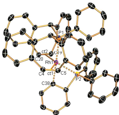
Figure 1. ORTEP plot (30% ellipsoid probability) showing the X-ray structure of 2 \cdot \frac{1}{2}\text{Et}_2\text{O} . The diethyl ether solvent molecule and hydrogen atoms have been omitted for clarity. Selected bond lengths ( \text{\AA} ) and angles (deg): Rh1–P1, 2.275(1); Rh1–P2, 2.382(1); Rh1–C38, 2.076(3); Rh1–C4, 2.185(3); Rh1–C5, 2.201(3); Rh1–C19, 2.171(3); Rh1–C20, 2.187(3); C4=C5, 1.414(3); C19=C20, 1.424(4); Rh1–ct1, 2.076(3); Rh1–ct2, 2.059(3); C38–Rh1–P1, 178.9(1); C38–Rh1–P2, 67.2(1); P1–Rh–P2, 113.9(1); ct1–Rh1–ct2, 132.9(1); \sum\angle(\text{C–P1–C}) , 310.9(4); \sum\angle(\text{C–P2–C}) , 319.7(4).
