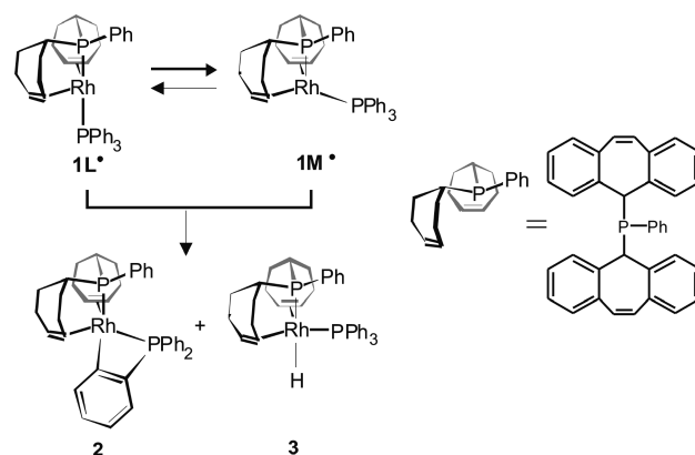
Scheme 2. Intermolecular C–H Bond Activation for 1L • / 1M •
