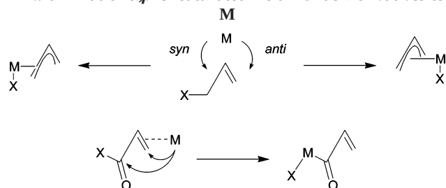
Scheme 2 Comparison of Oxidative Addition of Allyl-X to M with That of \alpha,\beta -Unsaturated Acid Halide Derivatives to M
