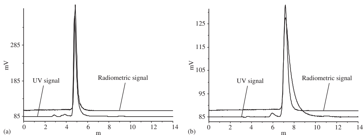
Figure 4. RP-HPLC chromatograms of [^{11}\text{C}]\text{-10} (A; \text{Rt} = 4.5 min) and [^{11}\text{C}]\text{-12} (B; \text{Rt} = 7.1 min) co-injected with their authentic non-radioactive analogues.
