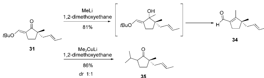
Scheme 3. Versatility of enol ether 31 .
