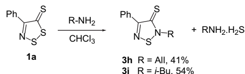
Scheme 2. Reaction of 4-phenyl-5 H -1,2,3-dithiazole-5-thione 1a with aliphatic amines.
