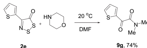
Scheme 9. Reaction of 5H-1,2,3-dithiazole-5-one 2e with morpholine in DMF.
