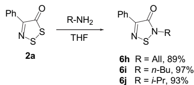
Scheme 4. Reaction of 4-phenyl-5H-1,2,3-dithiazol-5-one 2a with aliphatic amines.
