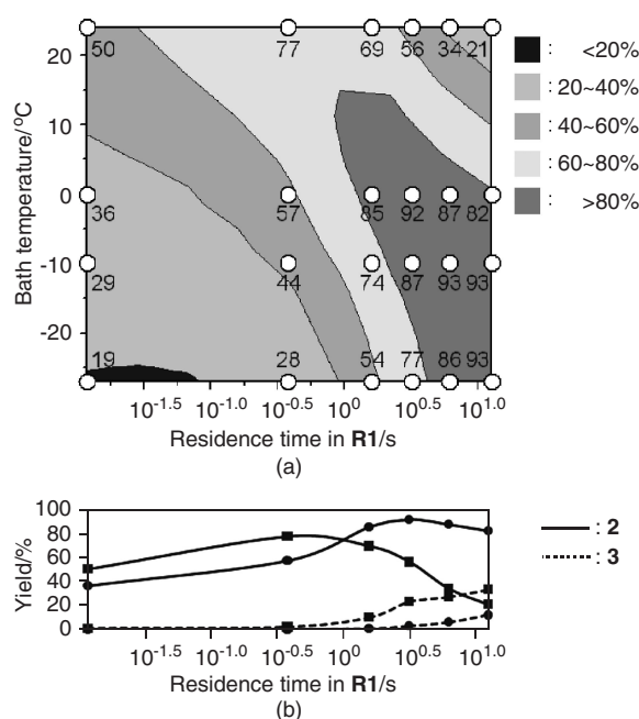
Figure 2. Effects of temperature and residence time on the yield of 1-trimethylsilyl-1-triphenylsilylperoxyethane ( 2 ): (a) Contour plot with scatter overlay of the yields (%). (b) The yields of 2 and 3 , Cross section at 0 and 24 °C (●: 0 °C, ■: 24 °C).
