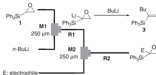
Figure 1. Microflow system for deprotonation of epoxyethyltriphenylsilane ( 1 ). T-shaped micromixer: M1 (inner diameter: 250 \mu m) and M2 (inner diameter: 250 \mu m), microtube reactor: R1 and R2 ( \phi = 1000 \mu m, length = 50 cm), a solution of epoxyethyltriphenylsilane: 0.10 M in THF (6.0 mL/min), a solution of n -BuLi: 0.60 M in hexane (1.5 mL/min), a solution of electrophile: 0.36 M in THF (3.0 mL/min).
