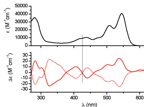
Figure 2. UV–vis absorption (top, identical for P - 2 and M - 2 ) and CD spectra (bottom) of P - 2 (solid red line) and M - 2 (dotted red line) enantiomers of PBI 2 in dichloromethane at 20\text{ }^\circ\text{C} .
