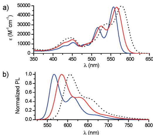
Figure 3. (a) UV–vis absorption and (b) normalized emission spectra of PBIs 3 (blue lines), 4 (red lines), and 5 (dotted lines) in dichloromethane at room temperature.
