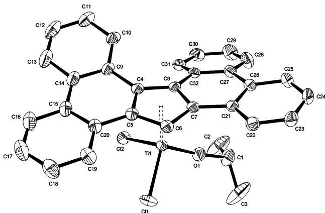
Figure 8. ORTEP plot of the solid-state molecular structure of 11 . Hydrogen atoms are omitted for clarity; thermal ellipsoids are drawn at the 50% probability level. Selected bond lengths [Å] and angles [deg]: Ti(1)–Ct(1) 2.049, Ti(1)–O(1) 1.733(3), Ti(1)–Cl(1) 2.284(9), Ti(1)–Cl(2) 2.285(7), O(1)–C(1) 1.426(3), C(4)–C(5) 1.417(3), C(4)–C(8) 1.446(3), C(5)–C(6) 1.422(3), C(6)–C(7) 1.416(3), C(7)–C(8) 1.423(3), Ti(1)–O(1)–C(1) 173.25(1), C(9)–C(4)–C(8)–C(32) 21.3(4).
