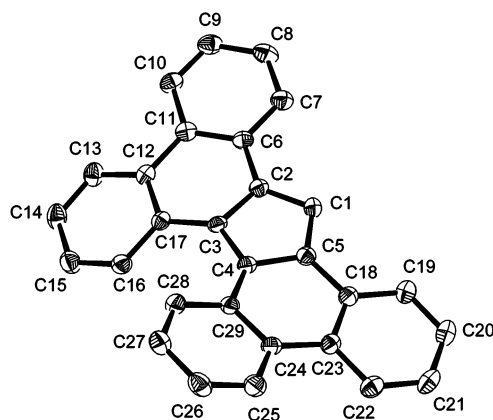
Figure 1. ORTEP plot of the solid-state molecular structure of 5 . Hydrogen atoms are omitted for clarity; thermal ellipsoids are drawn at the 50% probability level. Selected bond lengths [Å] and angles [deg]: C(1)–C(2) 1.404(3), C(1)–C(5) 1.406(3), C(2)–C(3) 1.431(3), C(3)–C(4) 1.431(3), C(4)–C(5) 1.425(3), C(17)–C(3)–C(4)–C(29) 30.4(4).
