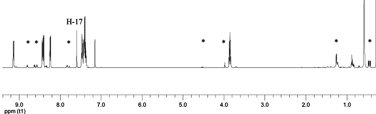
Figure 6. 1 H NMR spectrum (500.13 MHz, 300 K) of 10 in CDCl 3 (polar solvent) and C 6 D 6 (nonpolar solvent). The asterisks demark subsequent products.
