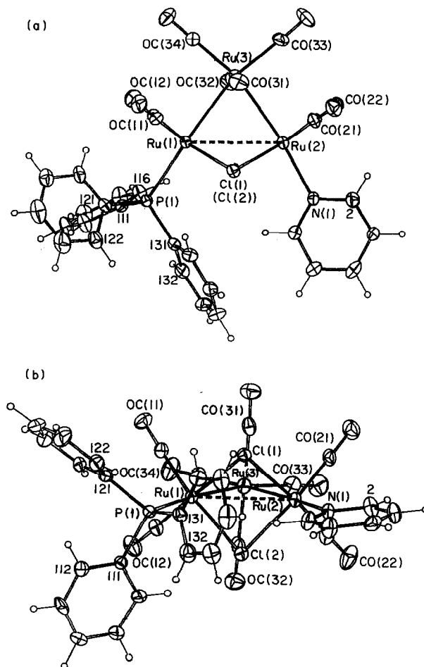
Fig. 2. Molecular structure and crystallographic numbering scheme for \text{Ru}_3(\mu\text{-Cl})_2(\text{CO})_8(\text{NC}_5\text{H}_5)(\text{PPh}_3) (6); 20% thermal ellipsoids are shown for the non-hydrogen atoms. Hydrogen atoms have arbitrary radii of 0.1 Å. Projections are shown (a) normal to and (b) oblique to the \text{Ru}_3 plane.
