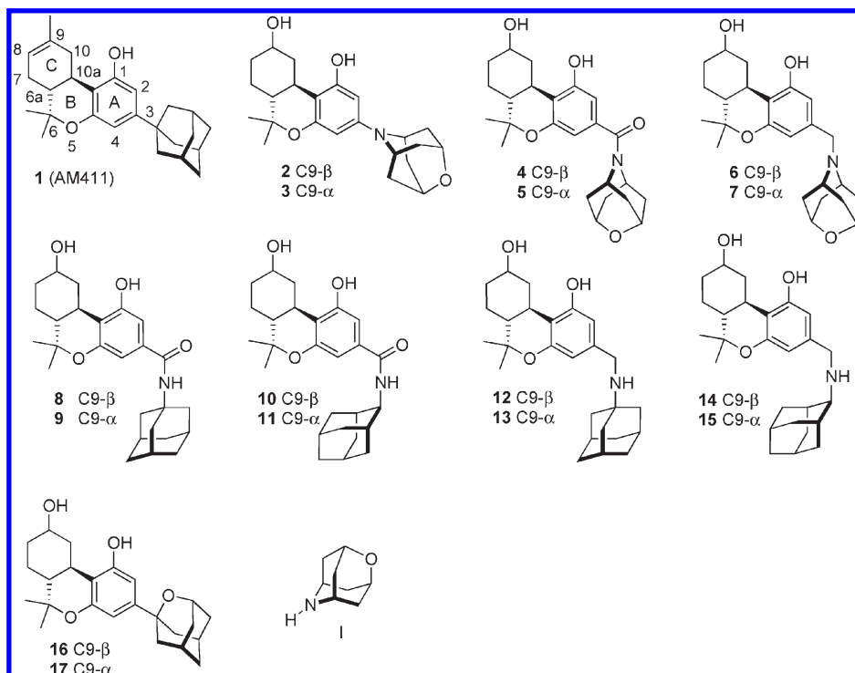
Figure 1. Adamantyl and heteroadamantyl cannabinoids.
