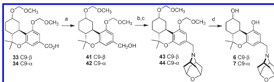
Scheme 2. Synthesis of Benzylamines 6 and 7 a
