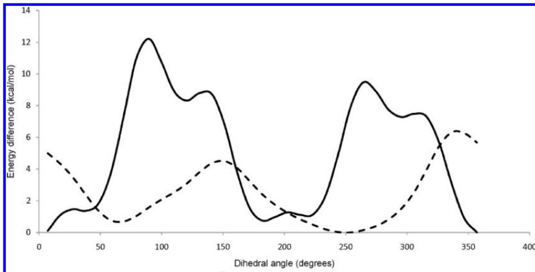
Figure 3. Plot of the QM energy relative to the lowest energy structure calculated at the B3LYP/6-31G** level for 16 (dashed) and 2 (solid) during a coordinate scan around the C3–C1' bond.
