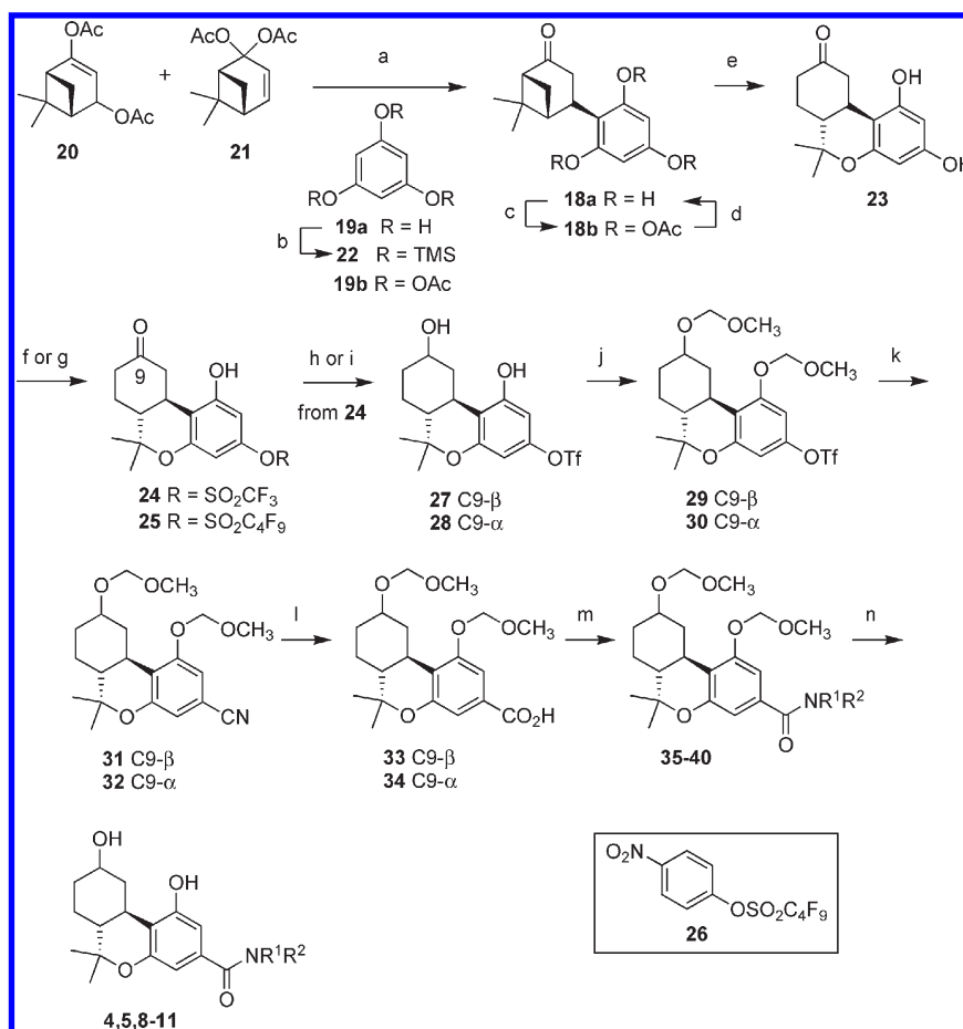
Scheme 1. Synthesis of Amides 4,5 and 8–11 a
