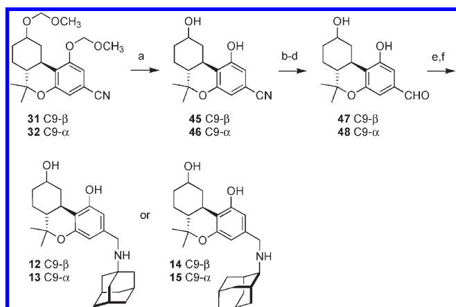
Scheme 3. Synthesis of Benzylamines 12–15 a
