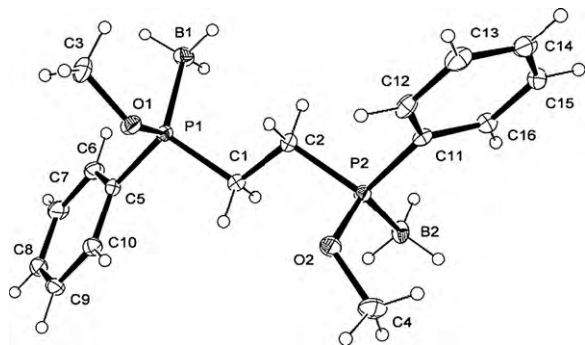
Fig. 3. Crystal structure of the ( S,S )-diphosphinite diborane 18 . Selected bond lengths (Å), angles (°): (a) P(1)–C(1) 1.806(3), P(2)–C(2) 1.804(3), P(1)–C(5) 1.803(3), P(2)–C(11) 1.805(3), P(1)–O(1) 1.607(3), P(2)–O(2) 1.600(2), P(1)–B(1) 1.895(3), P(2)–B(2) 1.889(4); O(1)–P(1)–C(1) 99.90(14), O(2)–P(2)–C(2) 99.42(13), O(1)–P(1)–C(5) 106.13(13), O(2)–P(2)–C(11) 105.77(14), O(1)–P(1)–B(1) 116.66(17), O(2)–P(2)–B(2) 116.19(16).
