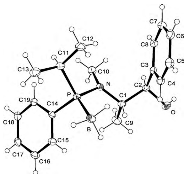
Fig. 2. Crystal structure of aminophosphine borane 12f with selected bond lengths (Å), angles (°): P–B 1.9206(19); P–N 1.6755(13), P–C(11) 1.8285(16), P–C(14) 1.8263(16); N–P–B 114.47(8); C(11)–P–B 112.31(8), C(14)–P–B 110.93(8), C(1)–N–P 118.35(10), C(1)–N–C(10) 116.03(13), C(10)–N–P 118.84(11).
