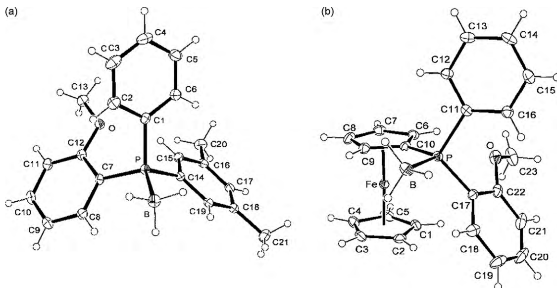
Fig. 1. Crystal structures: (a) Phosphine borane (R)- 15c . Selected bond lengths (Å), angles (°): P–B 1.917(2), P–C(1) 1.8138(18), P–C(7) 1.8170(17), P–C(14) 1.8165(16); C(1)–P–B 109.53(9); C(7)–P–B 111.37(8), C(14)–P–B 113.43(9). (b) Phosphine borane (R)- 15b . Selected bond lengths (Å), angles (°): P–B 1.913(3), P–C(10) 1.793(2), P–C(11) 1.815(2), P–C(17) 1.810(2), Cp(1)–Fe 1.659(2), Cp(2)–Fe 1.645(2); C(10)–P–B 109.87(12), C(11)–P–B 107.82(11), C(17)–P–B 112.83(13), Cp(1)–Fe–Cp(2) 176.86 (12).
