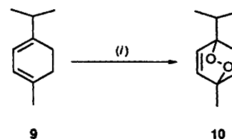
Scheme 2 (i) \text{H}_2\text{O}_2 -NaOH, 5 (1.5 mol%)
