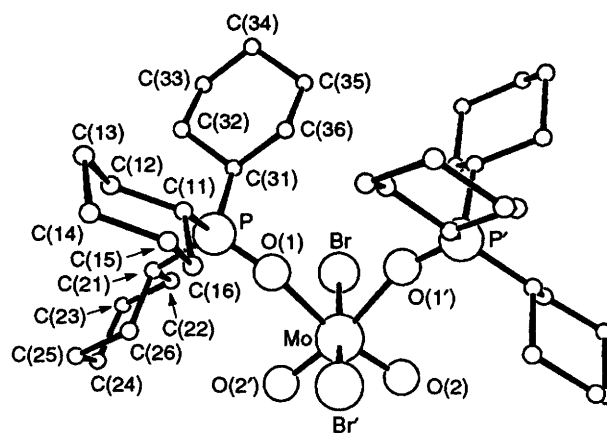
Fig. 3 An ORTEP representation of [\text{Mo}(\text{=O})_2\text{Br}_2\{\text{OP}(\text{C}_6\text{H}_{11})_3\}_2] 8 including the atomic numbering scheme but neglecting hydrogen atoms
