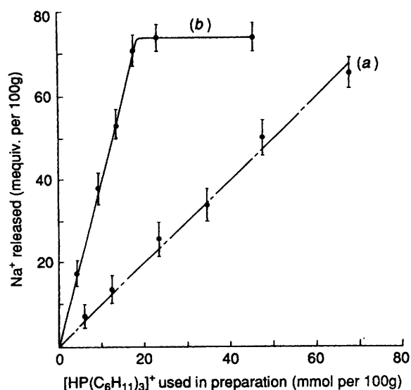
Fig. 2 A plot, with error bars, of \text{Na}^+ released/millimolar equivalents (mequiv.) per 100 g clay vs. [\text{HP}(\text{C}_6\text{H}_{11})_3]^+ used in preparation/mmol per 100 g clay for (a) preparations using [\text{HP}(\text{C}_6\text{H}_{11})_3]\text{Cl} and (b) preparations using [\text{HP}(\text{C}_6\text{H}_{11})_3][\text{Mo}(\text{=O})\text{Br}_4\{\text{OP}(\text{C}_6\text{H}_{11})_3\}]\cdot\text{C}_6\text{H}_5\text{Me} 5
