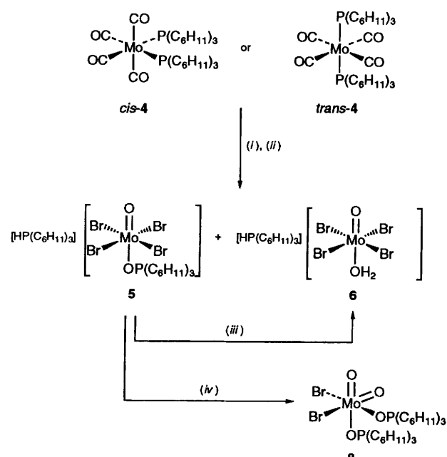
Scheme 1 (i) 1–2 equivalents \text{Br}_2 ; (ii) air, 6–10 days; (iii) 4\text{MeOC}_6\text{H}_4\text{OH} , water (trace); (iv) EtOH, 10 days
