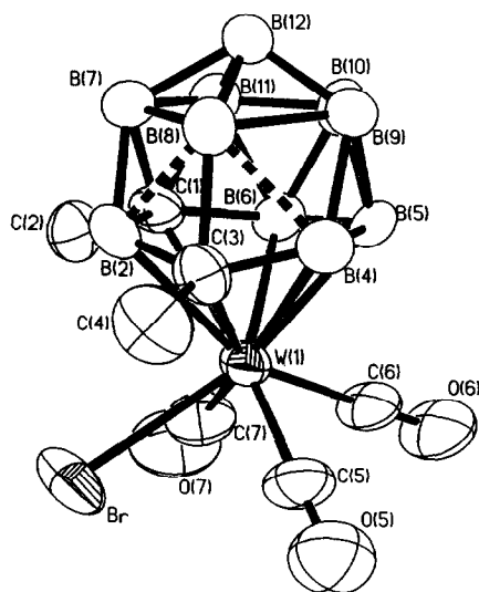
Fig. 1. ORTEP view of the anion of the salt [N(PPh_3)_2][WBr(CO)_3-(\eta^6-7,9-C_2B_9H_9Me_2)] ( 5b ), showing the crystallographic atom-labelling scheme. Thermal ellipsoids are shown at 50% probability level.
