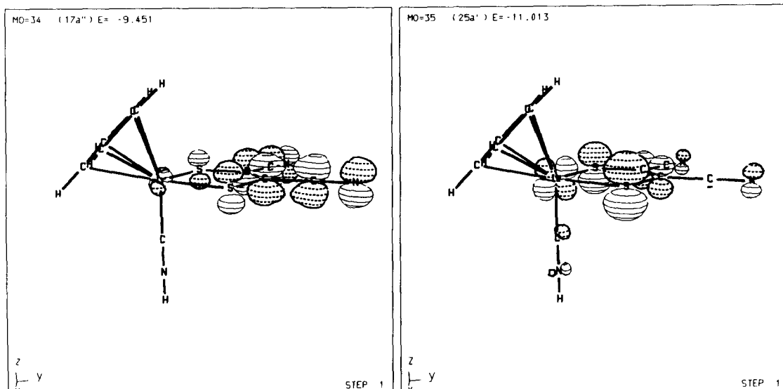
Fig. 3. CACAO drawings of the LUMO (left side) and the HOMO (right side) of (a) CpIr(PH 3 )(mnt) and (b) CpIr(CNH)(mnt).
