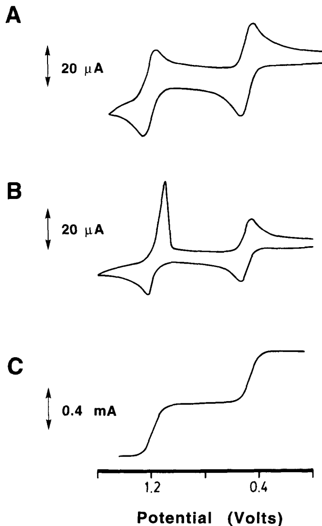
Fig. 2. Anodic scan cyclic voltammograms of ca. 1 \times 10^{-3} M \text{Cp}^+ \text{Ir}(\text{PMe}_3)_3(\text{mnt}) at room temperature containing 0.2 M TBAP at 0.5 V \text{s}^{-1} in (a) MeCN and (b) \text{CH}_2\text{Cl}_2 , and (c) rotating disc electrode voltammogram of ca. 1 \times 10^{-3} M \text{Cp}^+ \text{Ir}(\text{PMe}_3)_3(\text{mnt}) at room temperature in MeCN containing 0.25 M TBAP at 0.05 V \text{s}^{-1} .
