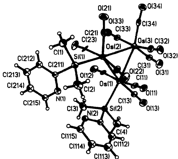
Fig. 1. The molecular structure of [\text{Os}_3(\mu\text{-H})_2(\text{CO})_{10}\{2\text{-(CH}_3)_2\text{-SiC}_5\text{H}_4\text{N}_2\}] showing the atom labelling scheme.
