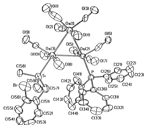
Fig. 3. The molecular structure of [\text{Os}_3(\mu\text{-H})(\text{CO})_{10}(\text{PPh}_3)\{2\text{-Br-C}_6\text{H}_4\text{CH}_2\text{Si}(\text{CH}_3)_2\}] ( 4 ) showing the atom labelling scheme.
