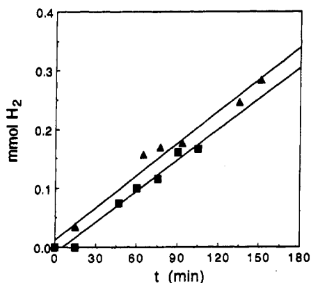
Figure 4. Hydrogen uptake measurements in the hydrogenation of (▲) quinoline and (■) DHQ to THQ by complex 4. [Rh] = 3.0 \times 10^{-4} M; [substrate] = 8.5 \times 10^{-2} M; [H_2] = 4.0 \times 10^{-3} M; solvent = toluene; V_{tot} = 50 mL; T = 373 K.
