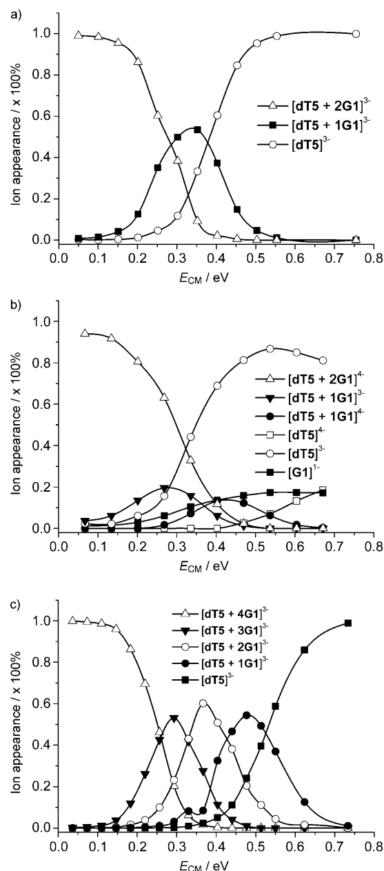
Figure 6. Ion-appearance plots for the CID experiments of a) [\text{dT5}+2\text{G1}]^{3-} ( m/z 780.92 \text{g mol}^{-1} ), b) [\text{dT5}+2\text{G1}]^{4-} ( m/z 585.45 \text{g mol}^{-1} ), and c) [\text{dT5}+4\text{G1}]^{3-} ( m/z 807.06 \text{g mol}^{-1} ) as a function of the collision energy, E_{\text{CM}} .
