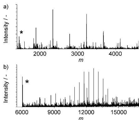
Figure 5. Deconvoluted ESI mass spectra for a) [G1] = 1 mM and [dT5] = 0.2 mM and b) [G1] = 1 mM and [dT20] = 0.05 mM in ultrapure water. * indicates the mass of the molecular ions for dT5 or dT20 , respectively.
