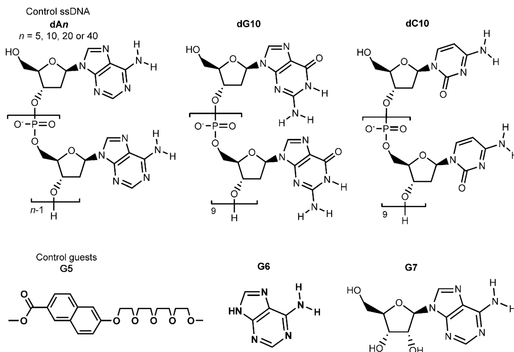
Scheme 2. Molecular structures of the control ssDNA and control guests.
